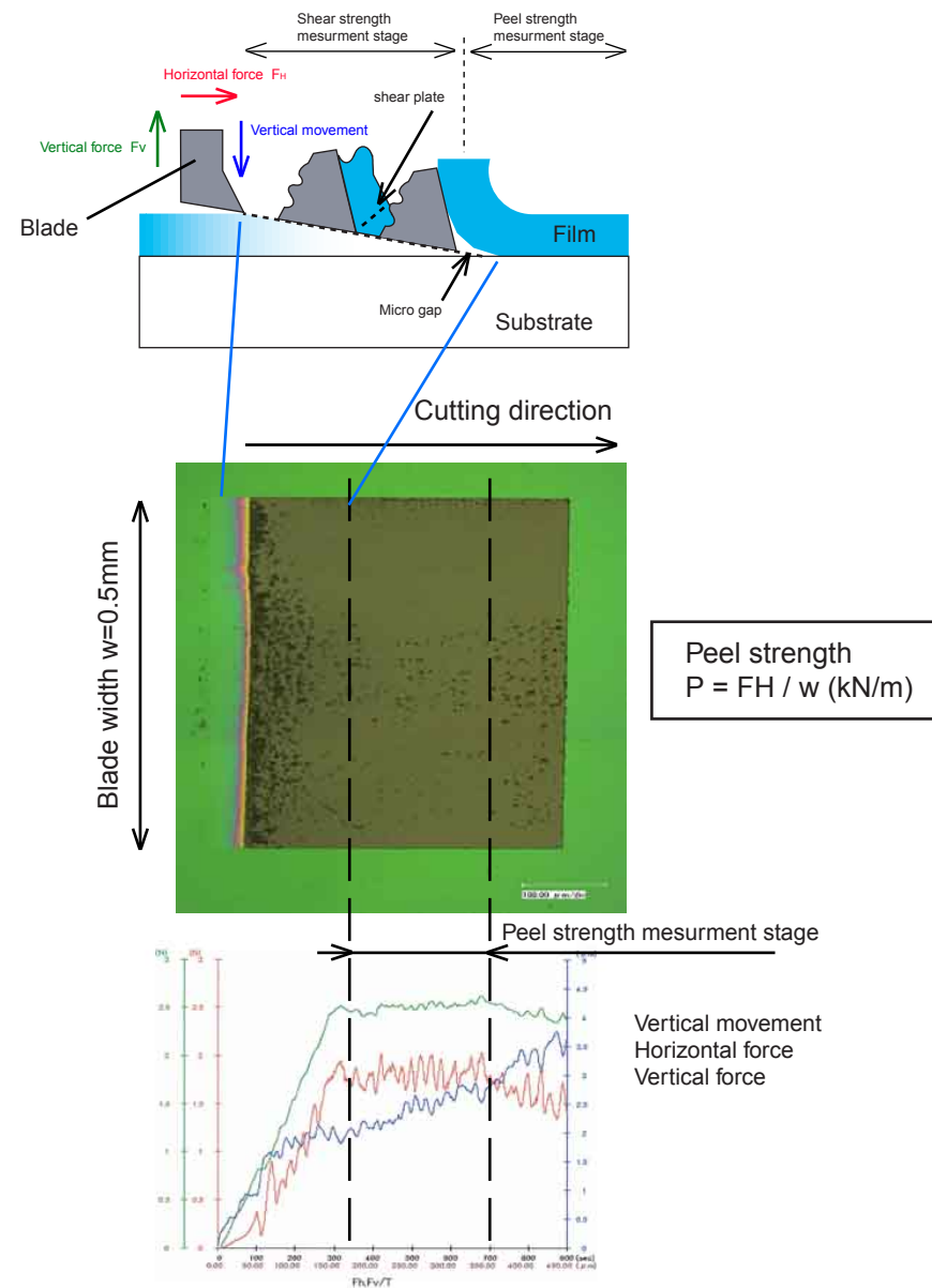
Surface And Interfacial Cutting Analysis System (SAICAS)
